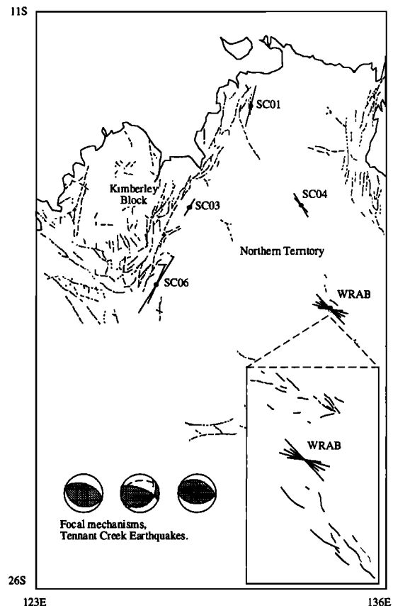
Figure 3. Polarization directions from high-frequency records of WRAB, SC01, SC03, SC04, and SC06 in relation to major crustal features (faults and thrusts). The inset shows detailed structural trends in the vicinity of WRAB and the focal mechanisms of the large Tennant Creek earthquakes of January 1988 (Bowman, 1992).
