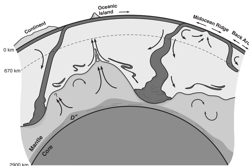
Fig. 1. Diagram illustrating the possible dynamics of an intrinsically dense layer in the lower mantle. Depth to the top of the layer ranges from \sim 1600 km to near the CMB, where it is deflected by downwelling slabs. Internal circulation within the layer is driven by internal heating and by heat flow across the CMB. A thermal boundary layer develops at the interface, and plumes arise from local high spots, carrying recycled slab and some primordial material.
