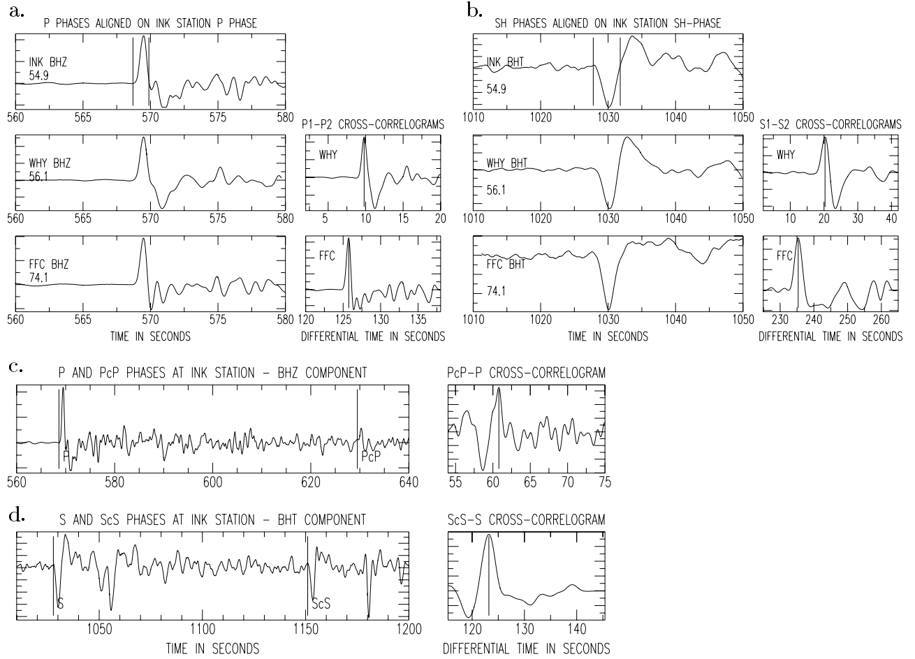
Figure 2. Example of data for an event on 20 July 2000 (latitude 36.4^{\circ}\text{N} , longitude 141.16^{\circ}\text{E} , depth 46 km, m_b = 6.1 ). (a) P_1 – P_2 differential travel time measurement using vertical components (BHZ). P wave is plotted for the reference station (top trace, station INK), and two other stations that have recorded the same event (middle and bottom left figures, stations WHY and FFC). Epicentral distance is written on each plot. The P wave first lobe of the reference trace, that is, the signal between the two vertical lines in the top plot, is cross-correlated with a window that contains P wave at the other stations. The differential travel time corresponds to the cross-correlogram maximum (vertical line on the cross-correlogram middle and bottom right plots). It is used for shifting data so that they get aligned to the reference station P wave for visual inspection. (b) S_1 – S_2 differential travel time measurement; same as Figure 2a but for S wave on transverse component (BHT). (c) PcP – P differential travel time measurement. The vertical seismogram (BHZ) is plotted on the left plot. The P wave first lobe is selected, modified using a t^* operator to account for differences in attenuation along the ray paths and cross-correlated with a window that contains the PcP phase. Differential travel time corresponds to cross-correlogram maximum (vertical line on the right plot), and it is reported on the seismogram with label PcP . (d) ScS – S differential travel time measurement; same as Figure 2c but for S wave on transverse components (BHT).
