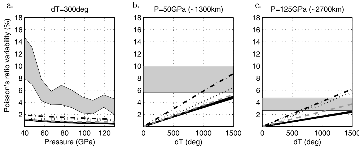
Figure 8. (a) Effect of a 300° thermal anomaly on Poisson's ratio at various pressures. Poisson's ratio perturbation is computed with equation (5) and the temperature-velocity derivatives of Stacey [1998] (dash-dotted line), Karato [1993] (dotted line), Trampert et al. [2001] (gray dashed line), and Karki and Stixrude [1999] (black line). For comparison, the gray area shows Poisson's ratio variability inferred from the range of acceptable models (same as Figure 7b except depth axis is converted to pressure). (b) and (c) Effect of various thermal anomalies on Poisson's ratio at a constant pressure of 50 GPa (~1300 km depth) (Figure 8b) and 125 GPa (~2700 km) (Figure 8c) using the same derivatives as in Figure 8a. Gray rectangle of Figures 8b and 8c shows Poisson ratio variability from our models at the given pressures.
