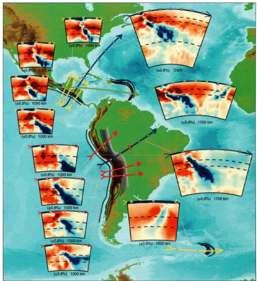
Plate 3. Cross-sections of a recent P -wave model [van der Hilst et al. , in preparation] to illustrate the likely complexity of slab structures. This model was obtained by inversion of travel time data from P , PP , pP , and several core phases ( PKP , Pdiff ), using an irregular grid parameterization, finite frequency sensitivity kernels [see also Kárason and van der Hilst, 2000], and corrections for crustal structure according to CRUST2.0 [http://mahj.ucsd.edu/Gabi/crust2.html]. The perturbations are shown in percent with respect to ak135 [Kennet et al. , 1995]. Negative anomalies are depicted by red colors and positive anomalies are in blue. The maximum scale is indicated below each cross-section together with its maximum depth. CMB, core–mantle boundary.
