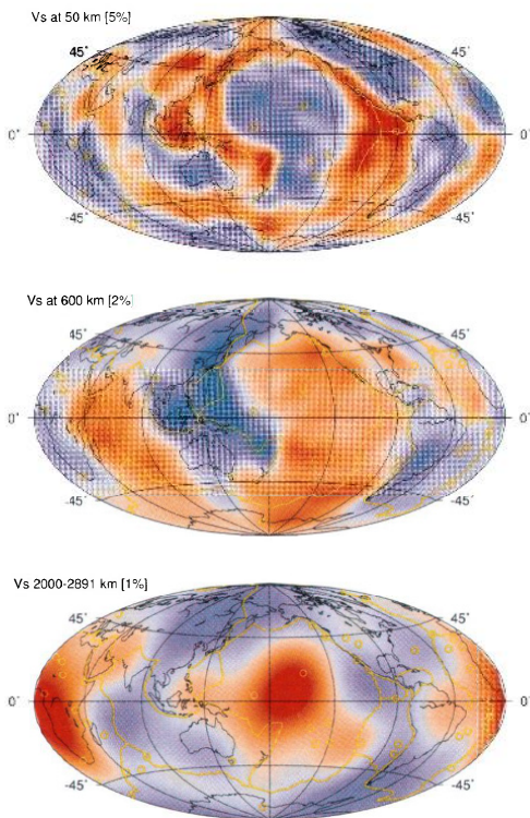
Plate 2. Models at 50- and 600-km depth obtained from the inversion of our fundamental and higher-mode surface wave phase velocity maps for variations in shear wave speed at a particular depth. The lowermost mantle layer is the most likely model from Trampert et al. [2004]. The perturbations are shown in percent variations with respect to PREM [Dziewonski and Anderson, 1981]. Negative wave speed anomalies are depicted by red colors and positive anomalies are in blue. The maximum scale is indicated beside each plot. The yellow lines indicate plate boundaries; yellow circles indicate hotspots.
