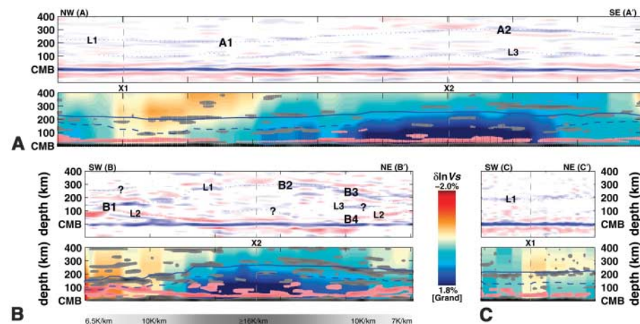
Fig. 3. Reflectivity from inverse scattering, at more than 75% confidence (18) (top) and S -speed ( \delta \ln V_s ) from tomography (19) (bottom). Scatter images are obtained by interpolation between GRT profiles (Fig. 1B, inset) calculated every 1° (~60 km at CMB) along sections A-A', B-B', and C-C' in Fig. 1. For the frequencies and incidence angles used, the radial resolution is ~10 km. The color scale for tomography is given between B-B' and C-C'. (A) L1, L2, and L3 label the scatter interfaces (thinly dashed). (B and C) The associated scatterers (visually enhanced) are superimposed on the tomography profiles, with dark gray depicting positive reflections and pink/red negative contrasts. Interface L1 aligns increases of wave speed with increasing depth; L2 delineates a decrease; L3 is more ambiguous but generally coincides with a wave-speed increase. Whereas L1 and L2 are piecewise continuous, L3 has an intermittent, en echelon appearance. The solid (dashed) blue lines in the bottom panels depict the phase transition location predicted by (21) (22). Points A1 and A2 and points B1 to B4 on L1 and L2 are used for temperature calculations (Fig. 4). The gray scale below B-B' depicts the lateral variation in temperature gradient along the CMB (for \gamma_{ppv} = 10 MPa/K) estimated from (29). In the central portion of the section, dT/dz cannot be determined directly because the occurrence of the double crossing cannot be resolved.
