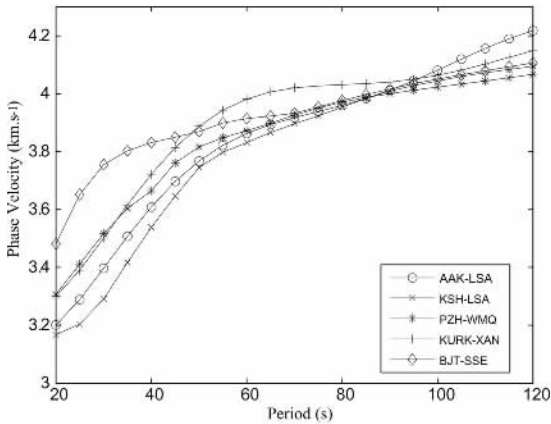
图3 5条不同双台路径上20~120s的Rayleigh波平均相速度频散曲线, 其台站位置请见图1 Fig.3 Average Rayleigh-wave phase velocity dispersion curves at periods 20~120s along 5 different inter-station paths. Please refer to Fig.1 about the location of stations illustrated here
