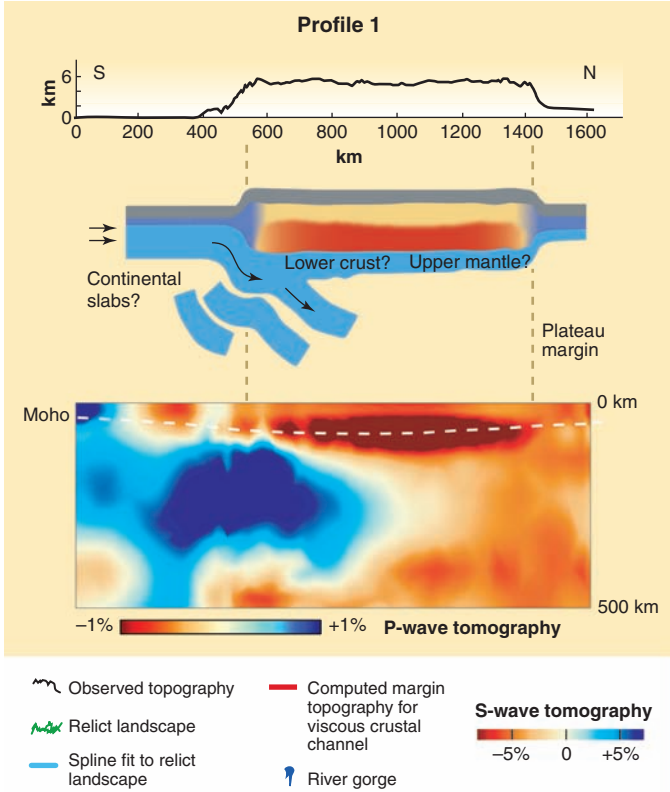
Fig. 5. Profiles through the Tibetan plateau region showing topography (top), conceptual crustal model (middle), and seismic section (bottom). Velocity anomalies are P -wave speed on profile 1 and S -wave speed on
