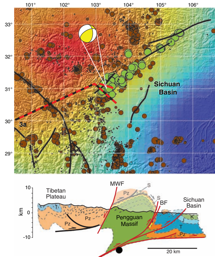
Fig. 6. (Top) Epicenters of 12 May 2008 Wenchuan earthquake and after-shocks (green circles), with focal mechanism for the main event (48). Events are superimposed on map of lateral variation in P -wave speed at 100-km depth relative to a laterally homogeneous reference Earth model (47), with color scale the same as in Fig. 4. Brown dots, regional seismicity (body wave magnitude larger than 3, symbol size scaled with magnitude, time interval 1964 to 2007) from EHB catalog (49). Map location given in Fig. 1. (Bottom) Geological structure along a profile through the hypocenter, modified after (28), with location shown by the red line on the map. Black lines, Jurassic faults; red lines, Late Cenozoic faults; S, Sinian (latest Proterozoic); MWF, Maowen-Wenchuan fault zone; BF, southern continuation of the Beichuan fault zone. Partially whited-out structures indicate geologic reconstruction above the modern topographic surface. Yellow circle depicts location of main Wenchuan earthquake with estimated uncertainty in depth of \pm 5 km.
